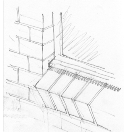
Example of bay window taken from local cottages showing the use of materials – facing brickwork and render splash course
