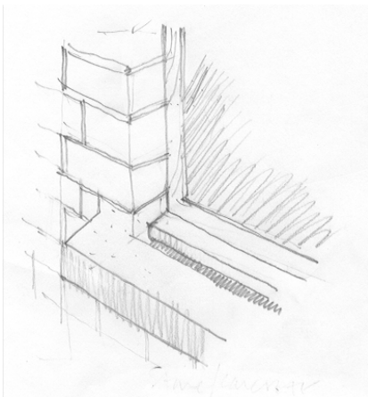
Stone cills using natural or reconstituted stone
